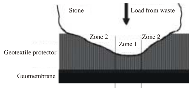
Figure 3. Stage 1 – Initial geotextile compression
