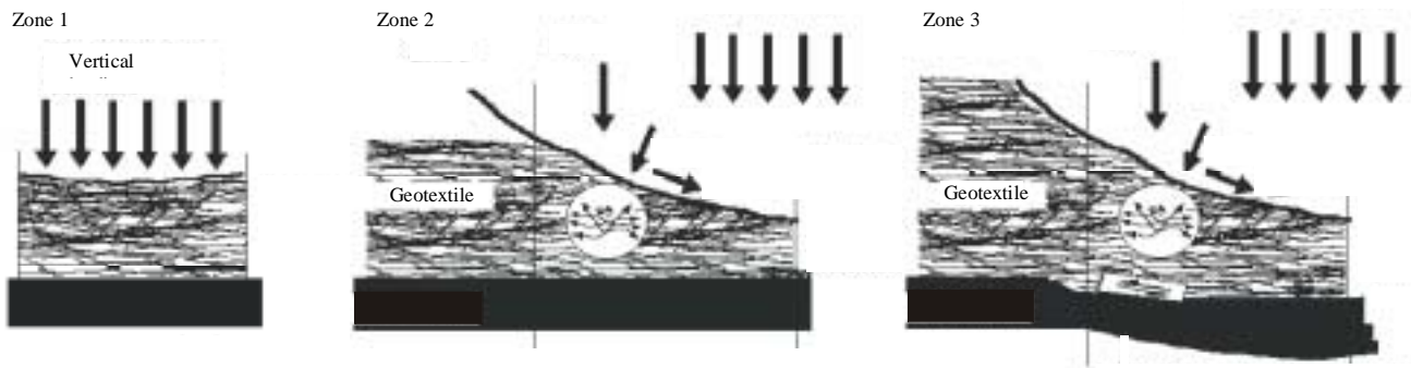
Figure 5. Schematic of the three zones of influence.
