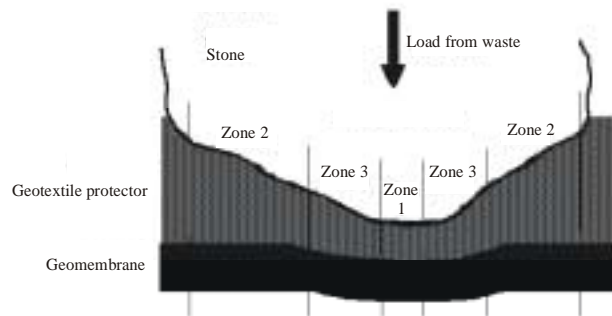
Figure 4. Stage 2 – Subsequent geotextile compression and geomembrane
